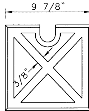
PLAN VIEW VALVE LID
