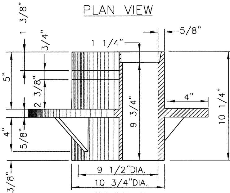
PROFILE VALVE BOX
