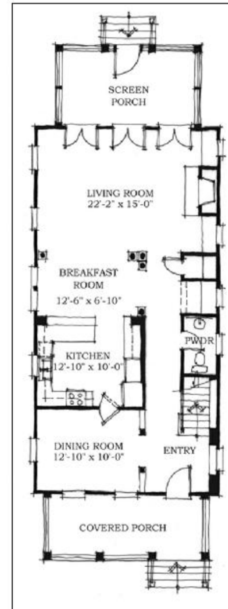
First Floor
