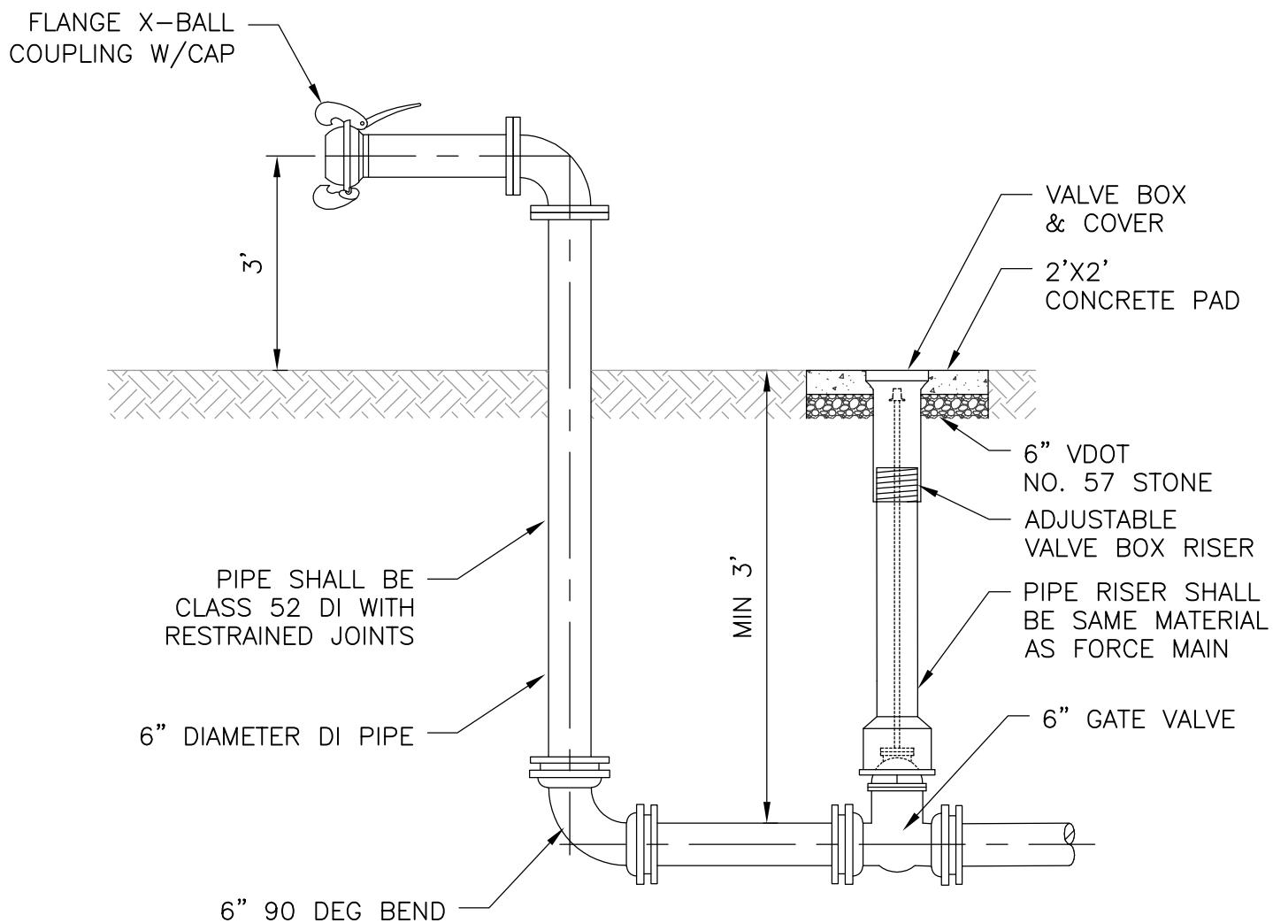
PROFILE
